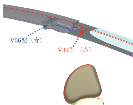
図-48 後席頭上空間の断面（側断面図） Fig. 48 Overhead clearance of rear seats (side view section)
